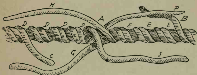
FIG. 107.—Long splice.
